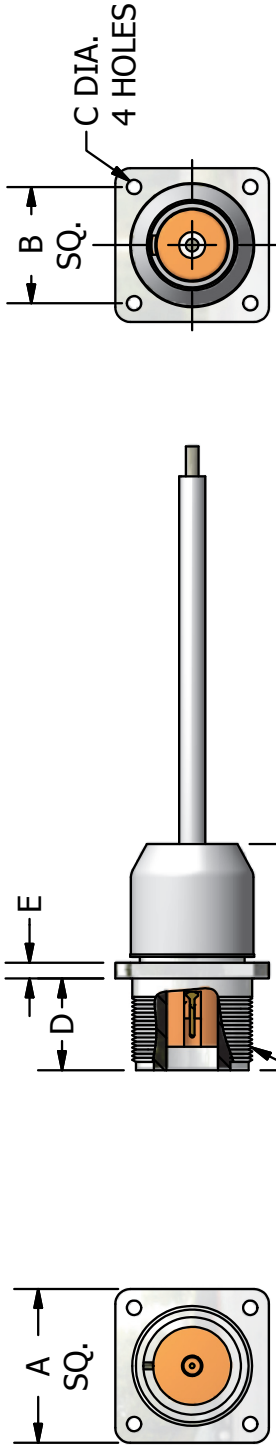
MOUNTING DIMENSIONS
